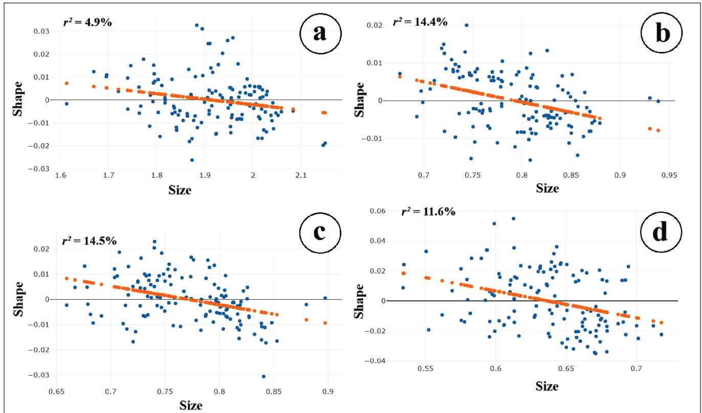
Figure 2. Wing allometric results, showing the relationships between the shape and size of four Lutzia species examined in this study for each wing element: (a) wing contour; (b) second submarginal cell; (c) first posterior cell; and (d) third posterior cell. Evaluations from the linear regression for predictions are indicated by orange dots, while blue dots represent individual samples.
