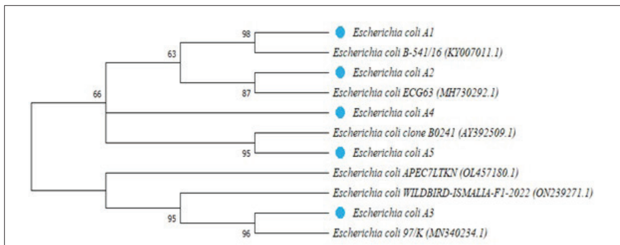
Figure 9. Phylogenetic tree of the fimH gene of E. coli isolates and E. coli strains retrieved from GenBank. Blue-chipped strains are from this study, while non-chipped strains are from GenBank retrievals.
