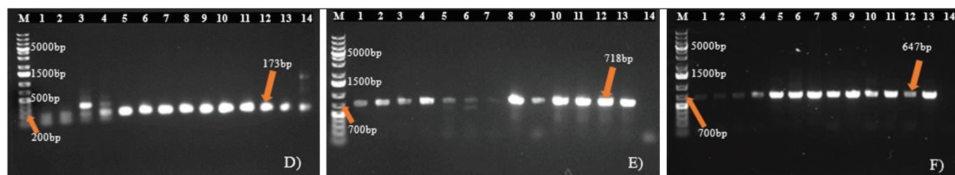
Figure 5. Agarose gel electrophoresis of amplified products for resistance genes in S. aureus (D) Gene bla Z (173 bp): M: Molecular ladder; 1-14: Positive samples; (E) Gene tet K (718 bp): M: Molecular ladder; 1-13: Positive samples; 14: Negative control; (F) Gene tet M (647 bp): M: Molecular ladder; 1-13: Positive samples; 14: Negative control.
