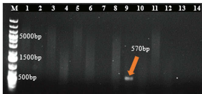
Figure 7. Agarose gel electrophoresis of amplified products for gene eae in E. coli (570 bp) M: Molecular ladder; 9: Positive sample; 1-8,10-13: Negative samples; 14: Negative control.
