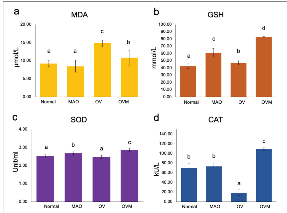
Figure 5. (a) MDA, (b) , (c) SOD, and (d)CAT activity in serum of hamsters in different groups: normal control, MAO, OV and OVM; in comparison to each experimental group p < 0.05 .
