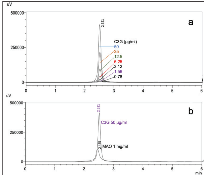
Figure 2. High-performance liquid chromatography analysis chromatogram. (a) C3G 0.78–50 µg/ml (b) C3G and MAO.
